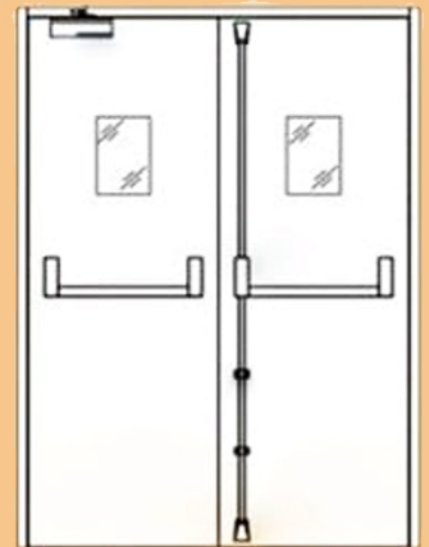
Double Leaf Fire Rated
