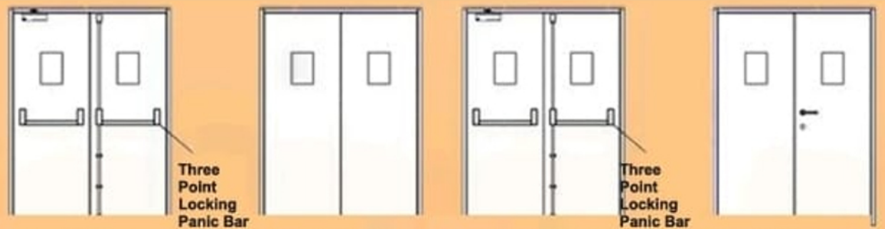
Front Elevation Back Elevation Double Leaf Fire-rated Door Without External Trim
