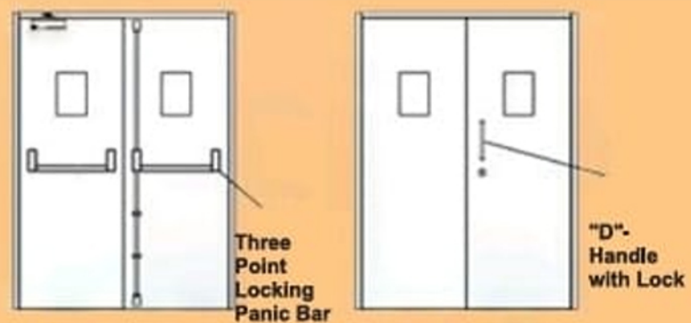
Front Elevation Back Elevation Double Leaf Fire-rated Door With External Trim (Option - II)
